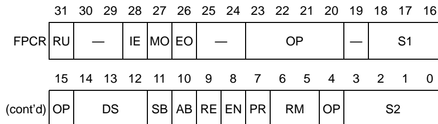
Figure 78.11 FPCR bit allocation in the FPA system
