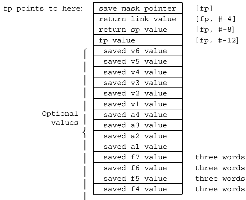
Figure 88.1 Stack backtrace data structure
