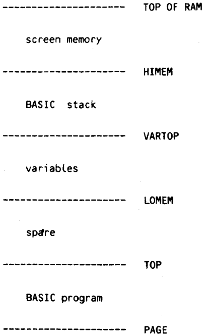
Figure 31. The BASIC program
