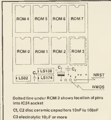
Figure 3. PCB layout
