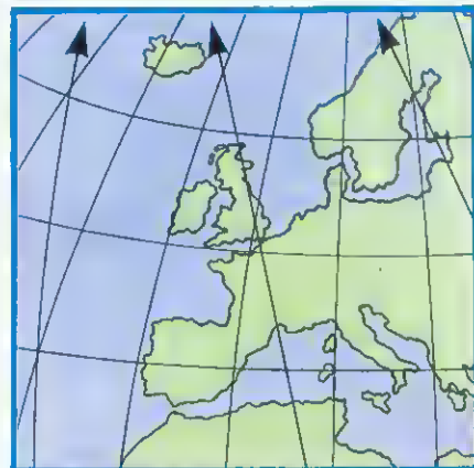
Figure 1. Consecutive orbits
