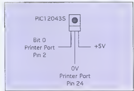
Figure II: An alternative infrared receiver
