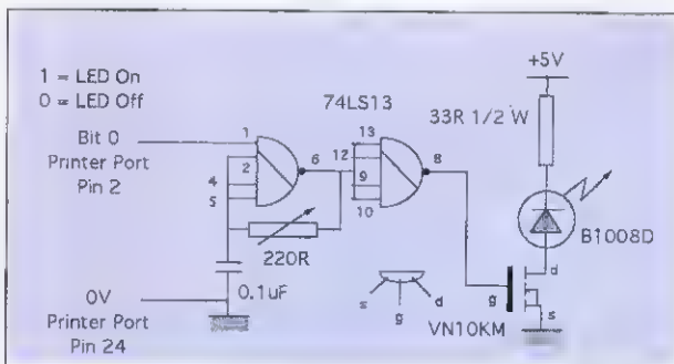
Figure III: The infrared transmitter circuit
