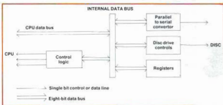
Figure 1. Overall structure of the 8271 chip
