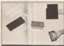
Figure 1. National Micro Centres' ROM extension socket system, consisting of extension cable with socket, ZIF socket, 'ashtray' aperture cover and sticky tape
