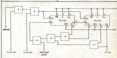
Figure 1. Hardware of the self-test signature analysis system
