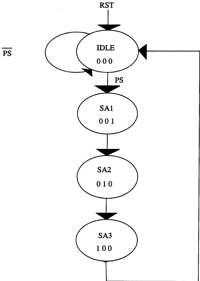
Figure 21.2 : State diagram
