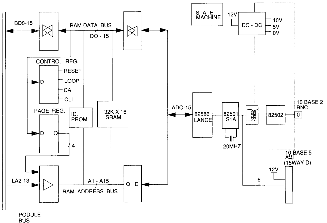
Figure 1: Ethernet I expansion card block diagram
