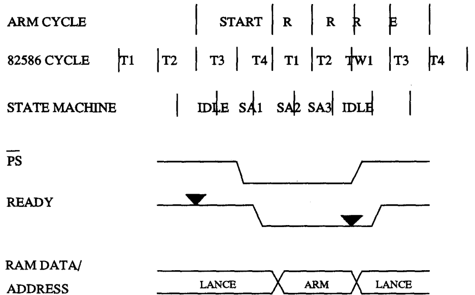
Figure 21.7 : Access collision cases - PS* while LANCE is in T4
