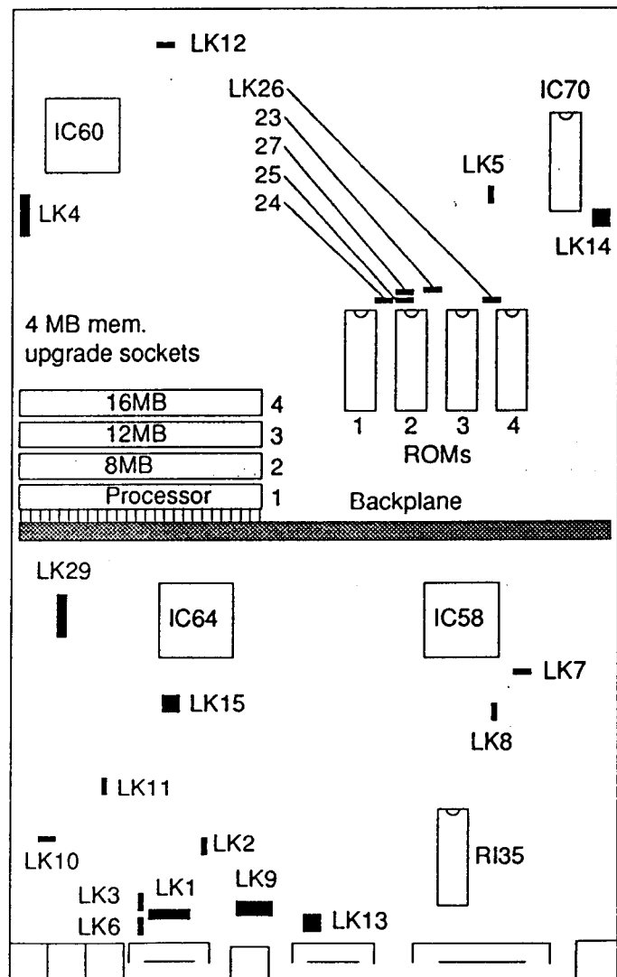
Fig 5-2: Link positions on main PCB
