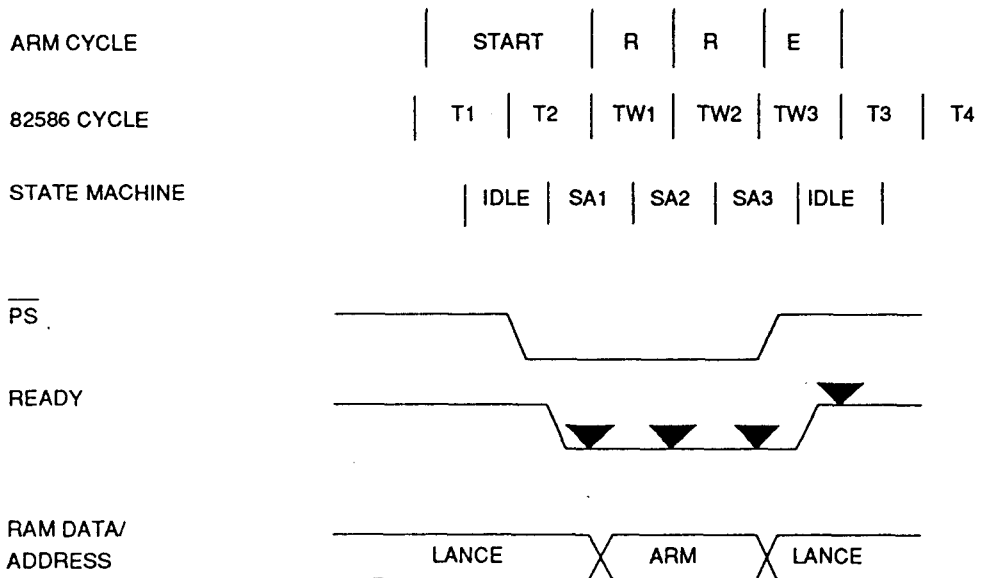
Figure 2-5: Access collision cases PS* while LANCE is in T2
