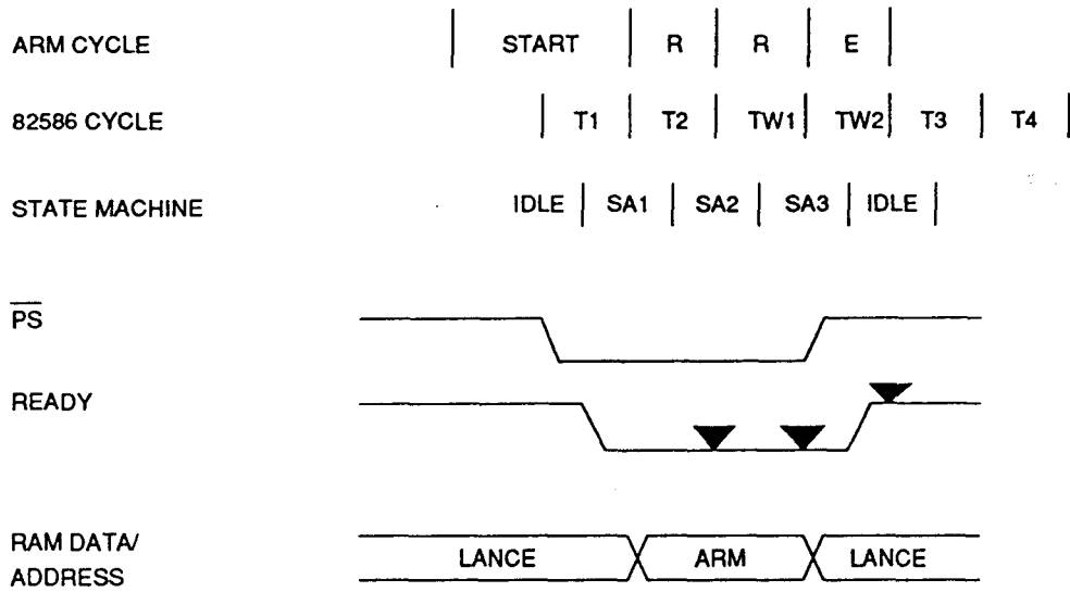
Figure 2-4: Access collision cases PS* while LANCE is in T1
