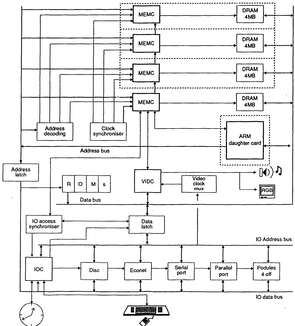
Fig 1-1: Block diagram of workstation
