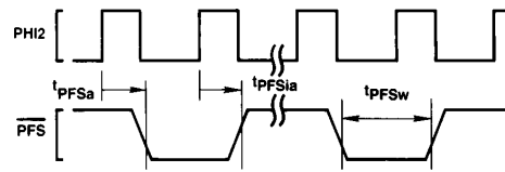
FIGURE 4-18. Relationship of \overline{\text{PFS}} to Clock Cycles
