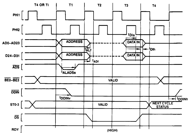
FIGURE 4-5. Read Cycle
