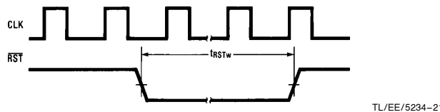
FIGURE 4-6. Non-Power-On Reset
