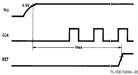
FIGURE 4-5. Power-On Reset
