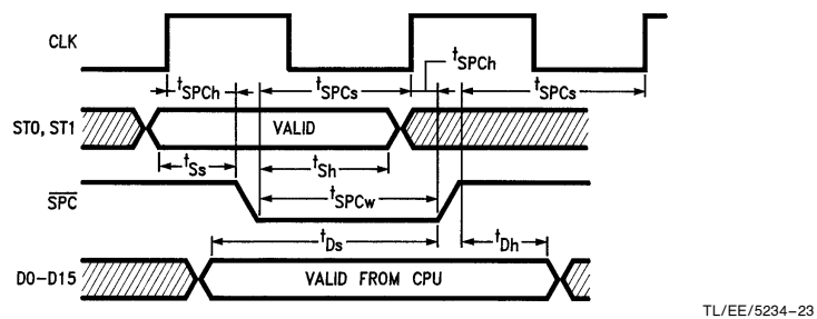
FIGURE 4-8. Write Cycle to FPU
